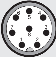
M12x1, 8 pole
