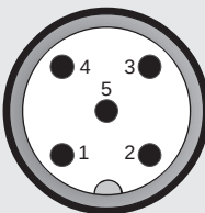
M12x1, 5 pole
