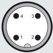
M12x1, 4 pole
